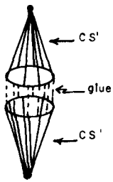
Fig. 5. Gluing together two copies of CS^1 along S^1 gives S^2 .
